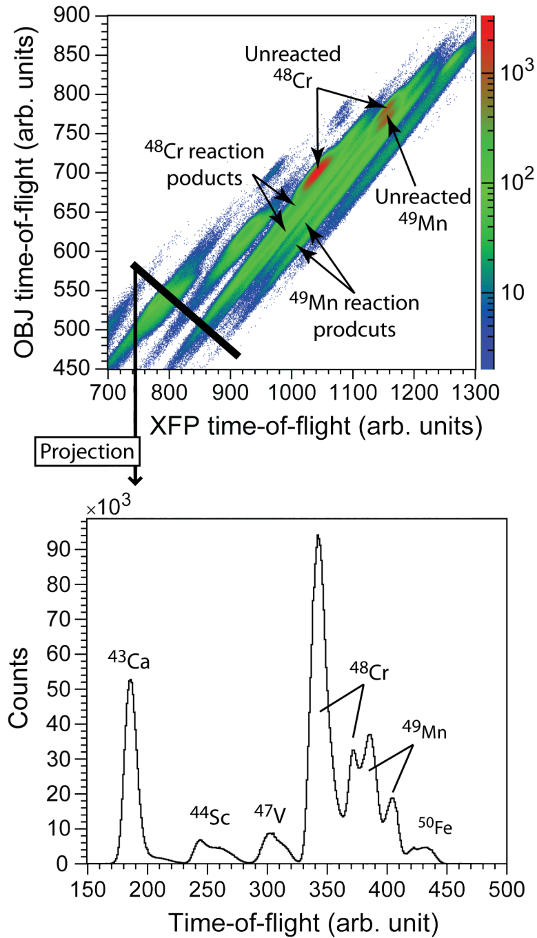
Figure 6.6: Time-of-flight broadening observed in the 9 Be pickup data. The runs summed above occurred after the addition of the delays but before the addition of the TACs. The top pane shows the two-dimensional histogram of XFP versus OBJ time-of-flight; the bottom pane is their difference. See Table 6.2 for the list of TOF definitions. The addition of the new electronics resolved the TOF broadening. See Figure 6.5.
