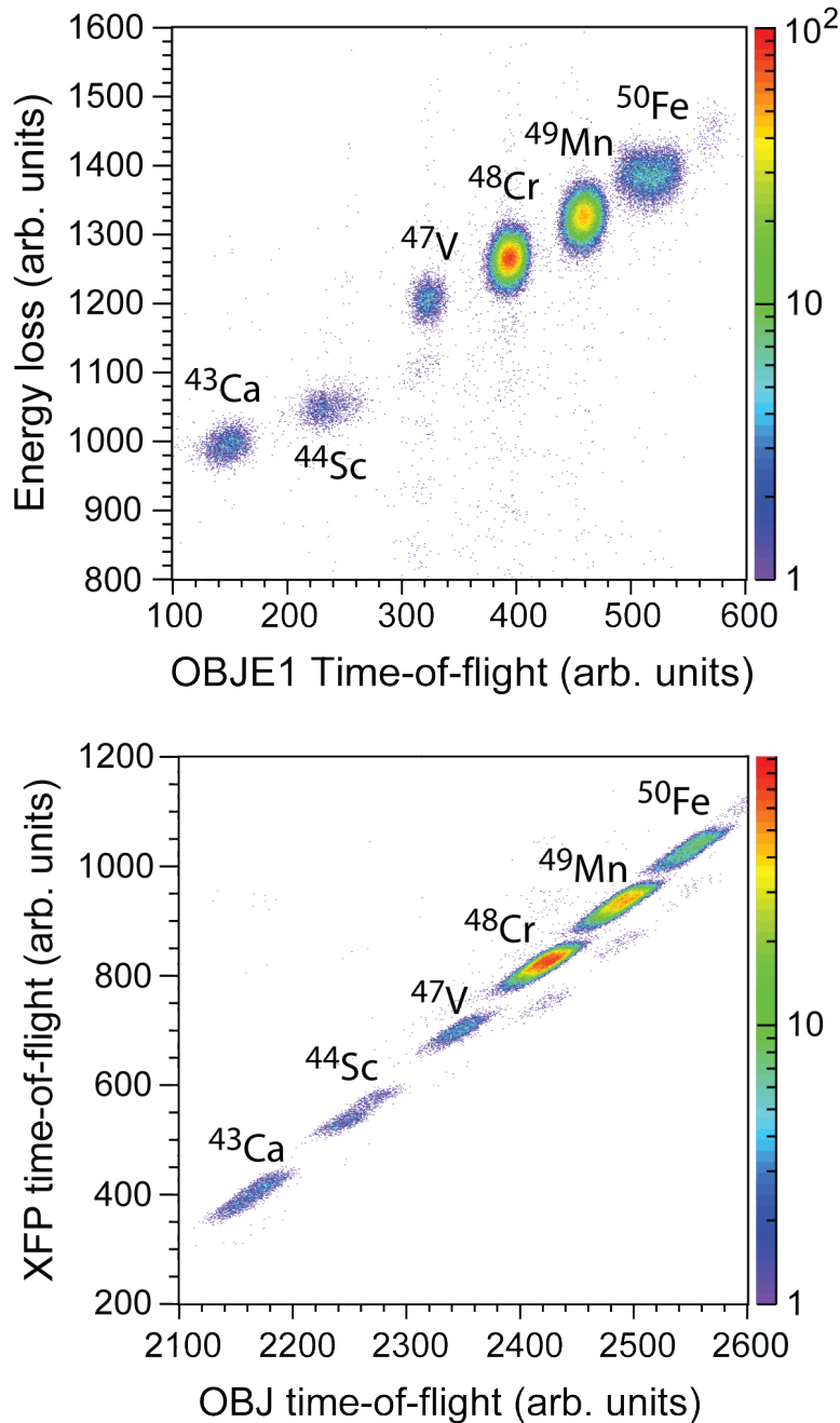
Figure 6.2: Particle identification spectra for an unreacted run (components of the incident cocktail projectile beam are centered in the focal plane) on the ^{12}\text{C} target showing the composition of the incoming cocktail beam. The upper pane shows a standard S800 PID plot of the TOF between the object scintillator (OBJ) and the back of the S800 focal plane (E1 scintillator) versus energy loss in the focal plane ion chamber. See Table 6.3 for a description of the OBJ, XFP, and OBJE1 labels given to the different TOF measurements. The lower pane is a two-dimensional TOF spectrum of XFP versus OBJ time-of-flight that can be used, like the one-dimensional difference spectrum shown in the bottom panel of Figure 6.4, to select a single component of the incoming cocktail beam.
