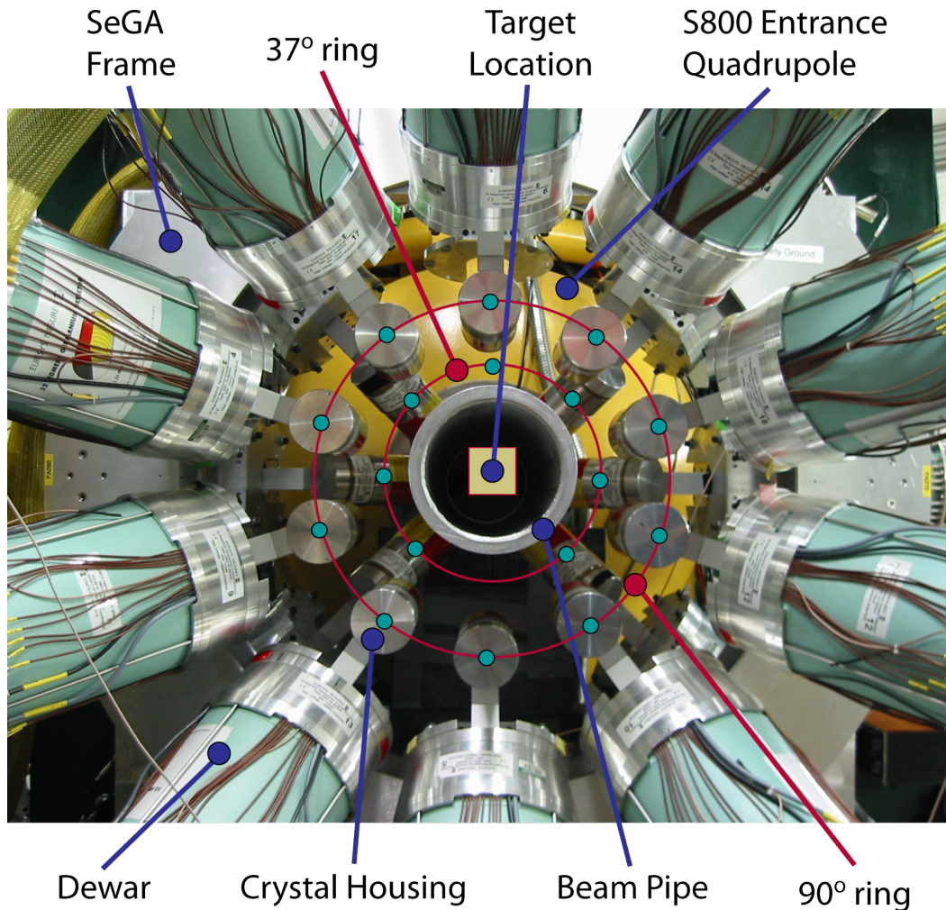
Figure 4.7: Photograph of the SeGA array in its “classic” configuration from a viewpoint upstream of the target position. Key components are labeled: the dewar and crystal housing for a single SeGA detector, the mounting ring, the 37° (7 detectors) and 90° rings (10 detectors), target location, 6in diameter beam pipe, and the yellow entrance quadrupole to the S800 spectrograph. In the photograph one detector is missing from the forward ring (the only aqua circle that does not tag a crystal housing). This detector was present for both experiments run in this thesis.
