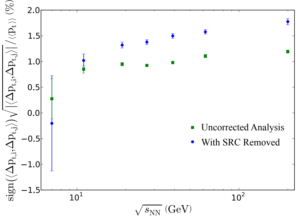
Figure 6.10: \text{sign}(\langle \Delta p_{t,i}, \Delta p_{t,j} \rangle) \sqrt{|\langle \Delta p_{t,i}, \Delta p_{t,j} \rangle| / \langle p_t \rangle} as a function of \sqrt{s_{NN}} with and without the short range correlation correction for the 0-5% centrality bin. The error bars are statistical errors. This observable is equivalent to \sqrt{\langle \Delta p_{t,i}, \Delta p_{t,j} \rangle / \langle p_t \rangle} , but the sign of \langle \Delta p_{t,i}, \Delta p_{t,j} \rangle is moved outside of the square root.
