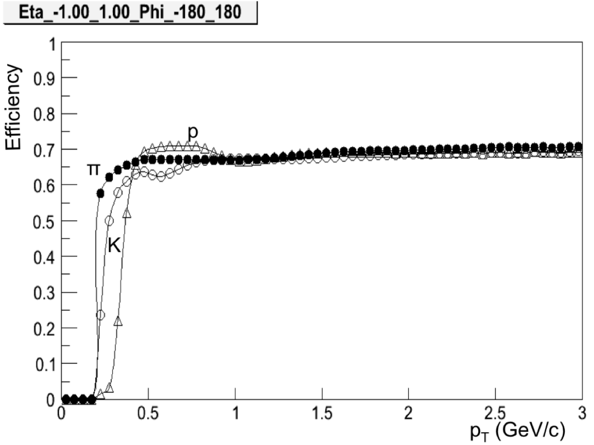
Figure 2.8: ToF matching efficiency for identified particle species. From Ref. [1].
