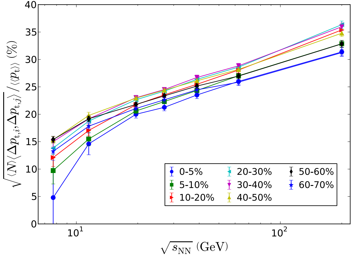
Figure 5.8: \sqrt{\langle N \rangle \langle \Delta p_{t,i} \Delta p_{t,j} \rangle / \langle \langle p_t \rangle \rangle} vs \sqrt{s_{\text{NN}}} for all seven energies and eight centrality bins. The error bars are statistical.
