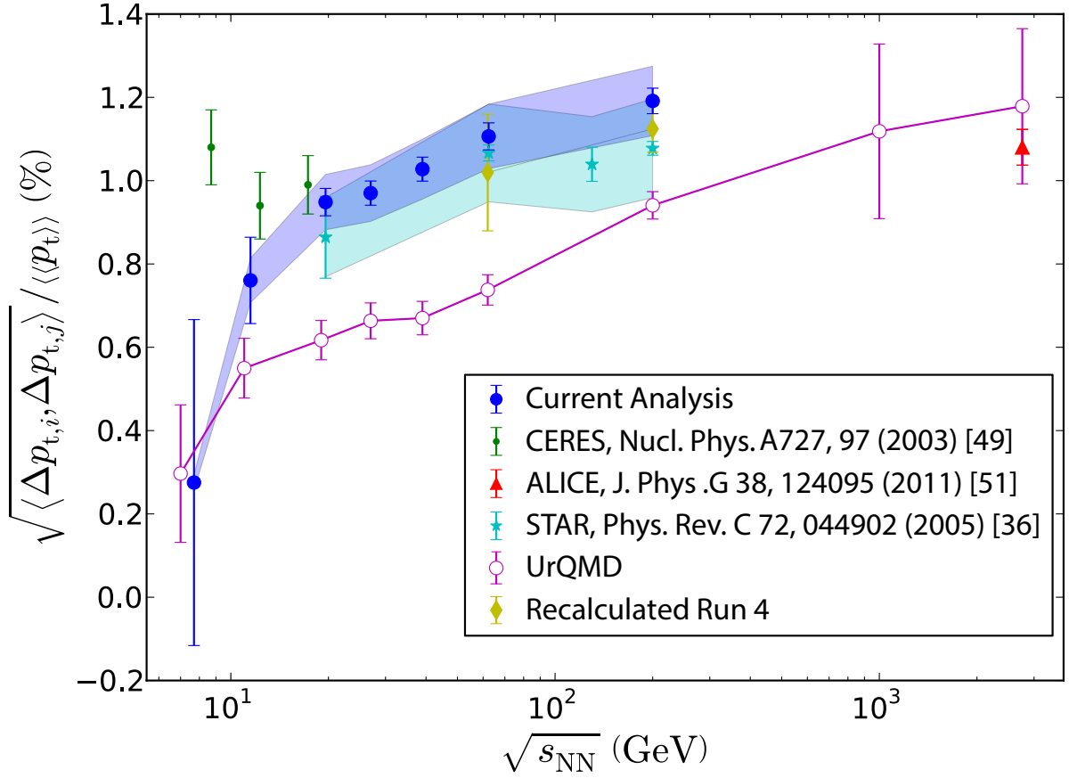
Figure 5.9: \sqrt{\langle \Delta p_{t,i} \Delta p_{t,j} \rangle} / \langle \langle p_t \rangle \rangle vs \sqrt{s_{NN}} for the 0-5% centrality bin for the present analysis and several other analyses. The error bars are statistical errors. The error bands are the systematic error of the STAR analyses.
