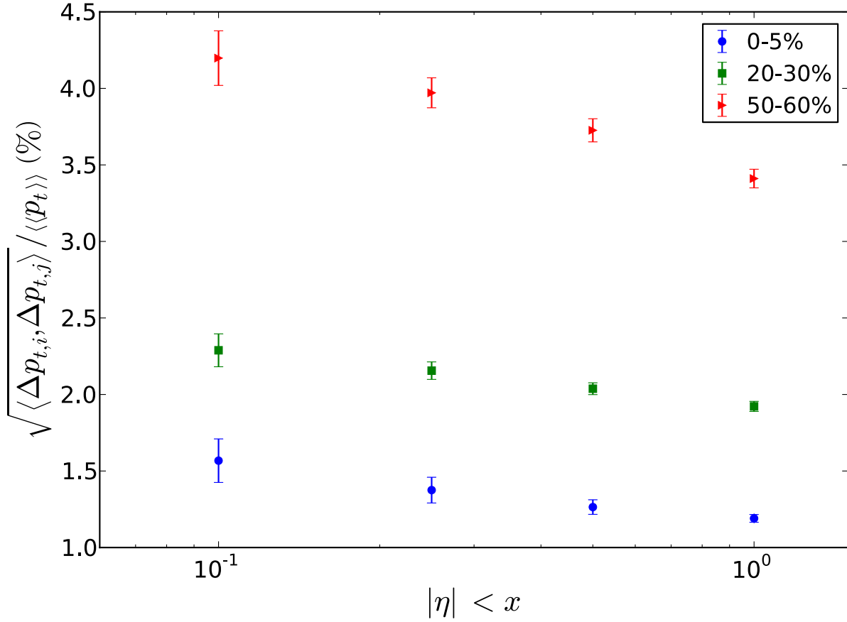
Figure 6.2: Comparisons of \sqrt{\langle \Delta p_{t,i} \Delta p_{t,j} \rangle} / \langle p_t \rangle calculated using different \eta cuts for 200 GeV. In all cases the \eta cut was symmetric about \eta = 0 . Three centrality bins are shown: 0-5%, 20-30%, and 50-60%. The error bars are statistical.
