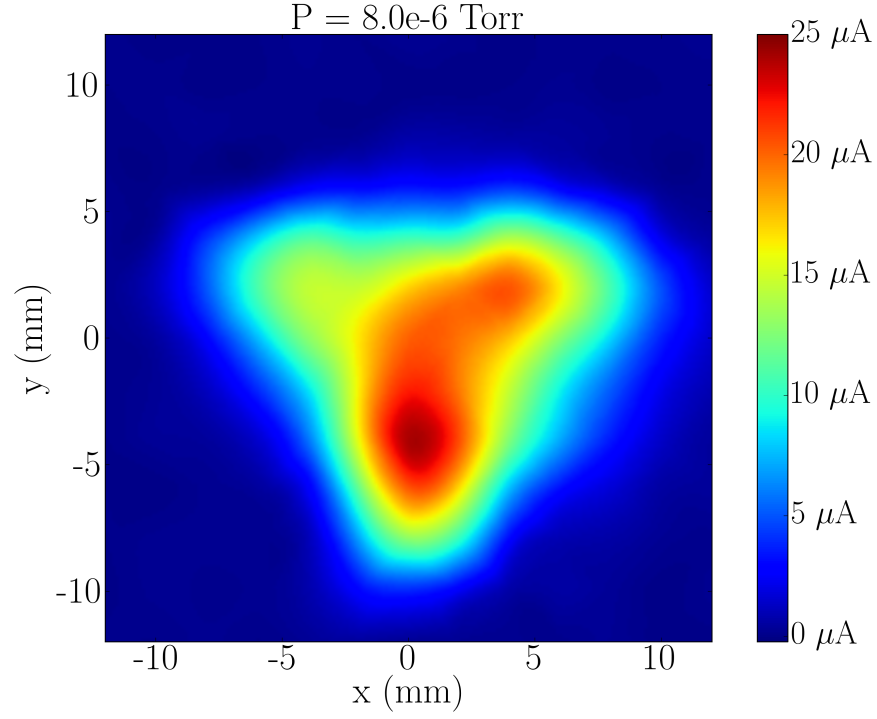
Figure 4.11: Example beam profile of an O^{3+} beam, \approx 235 e \mu A . The beam exhibits a triangular structure, which is typical for many ECRIS beams.
