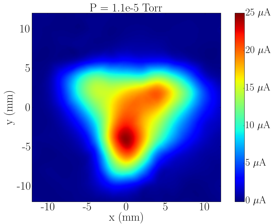
Figure 6.17: Measured beam profile of \text{O}^{3+} , 1.1 \cdot 10^{-5} Torr
