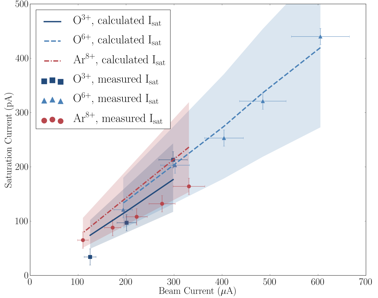
Figure 5.47: Saturation currents for three beam current variations in the SuSI LEBT at Q014. A transmission factor of T = 0.65 was used. The lower measured saturation current for the Ar^{8+} series could be due to the vertical asymmetry.
