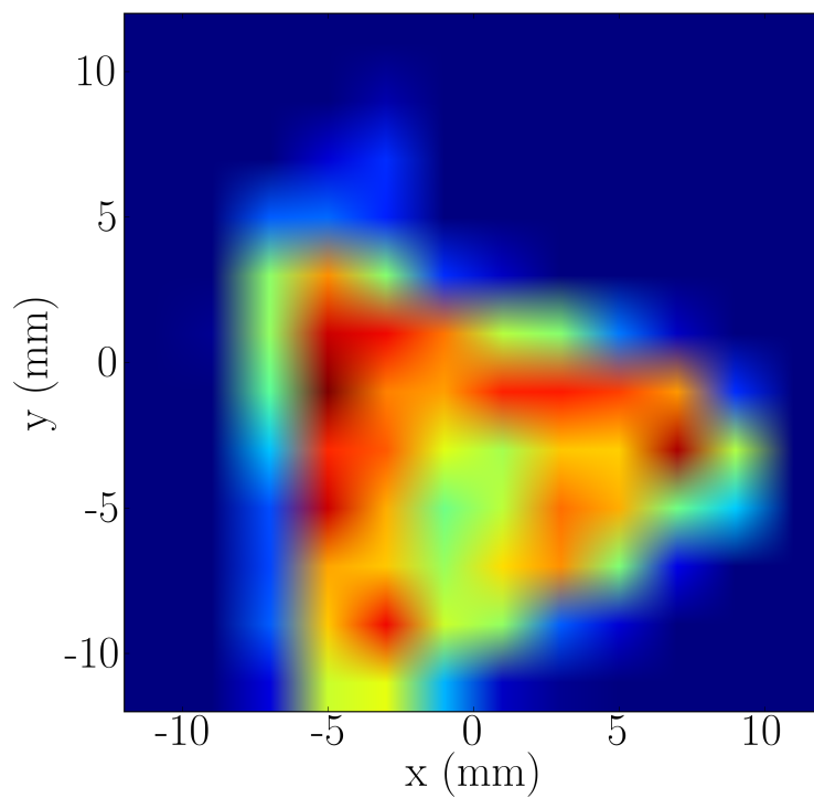
Figure 6.18: Simulated beam profile of \text{O}^{3+} , 1.1 \cdot 10^{-5} Torr
