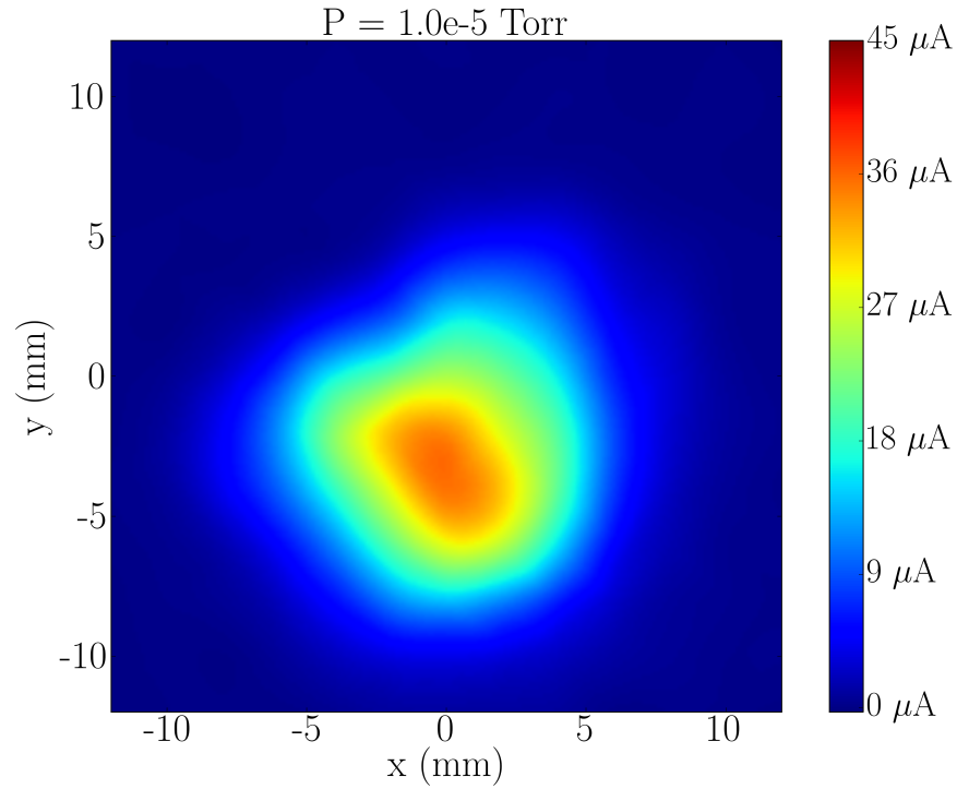
Figure 4.12: Example beam profile of an Ar^{8+} beam, \approx 200 e \mu A , tuned for 'roundness'.
