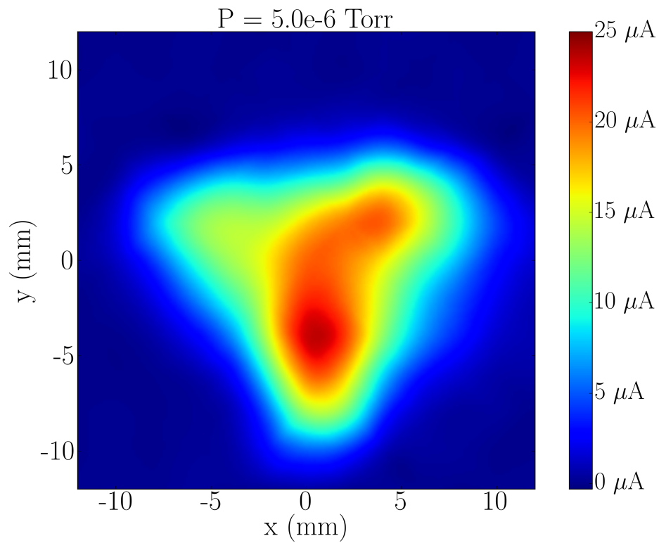
Figure 6.13: Measured beam profile of O^{3+} , 5.0 \cdot 10^{-6} Torr
