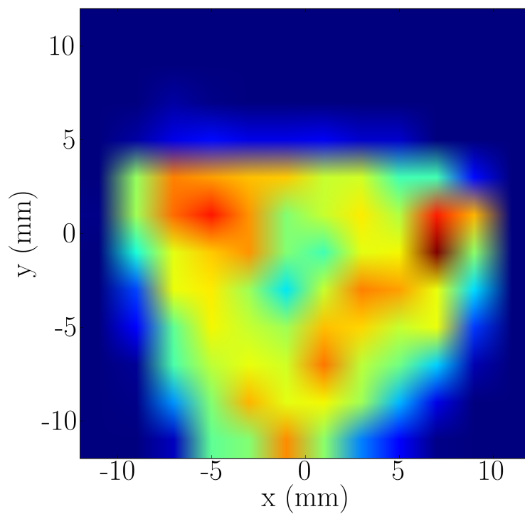
Figure 6.14: Simulated beam profile of O^{3+} , 5.0 \cdot 10^{-6} Torr
