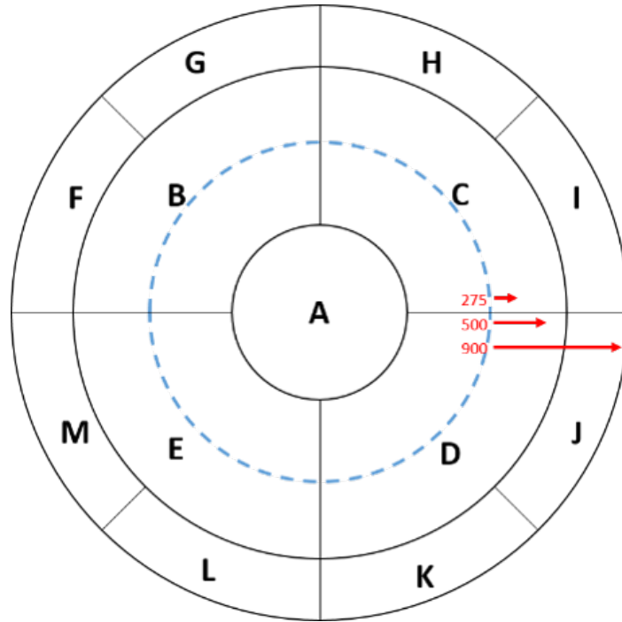
Figure 3.3: Diagram of the detector pad plane. The MICROMEAS is segmented into 13 charge-sensitive pads labeled A-M. The dashed blue circle represents the projection of the beam entrance window onto the pad plane, and the red arrows correspond to proton tracks. The size of the arrows, labeled by their energies in units of keV, are scaled in proportion to their calculated ranges in P10 gas at a pressure of 800 Torr.
