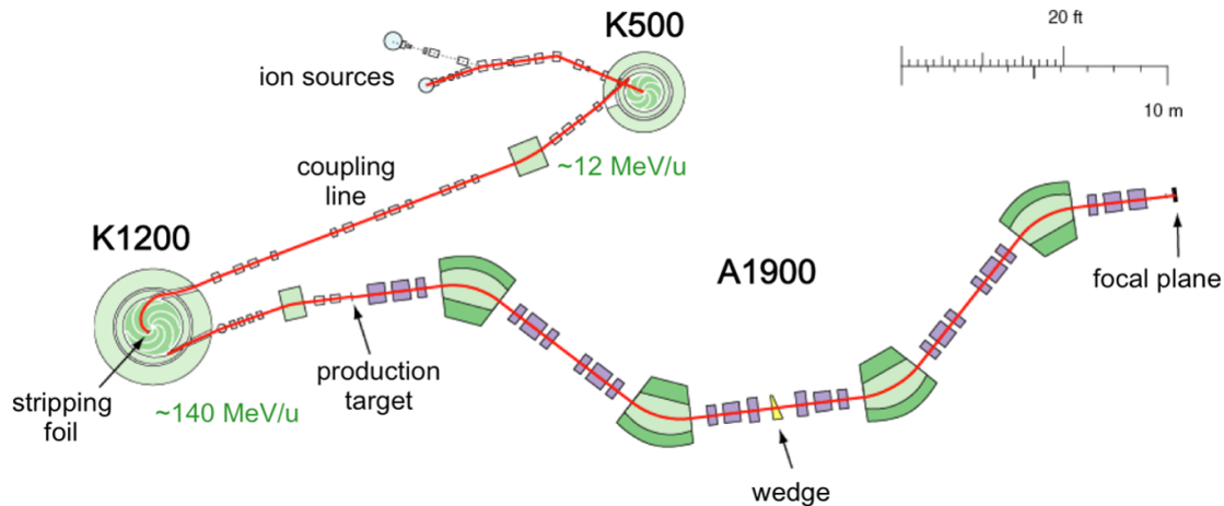
Figure 3.9: Diagram of the Coupled Cyclotron Facility and A1900 fragment separator at NSCL. Figure credit: Ref. [130].
