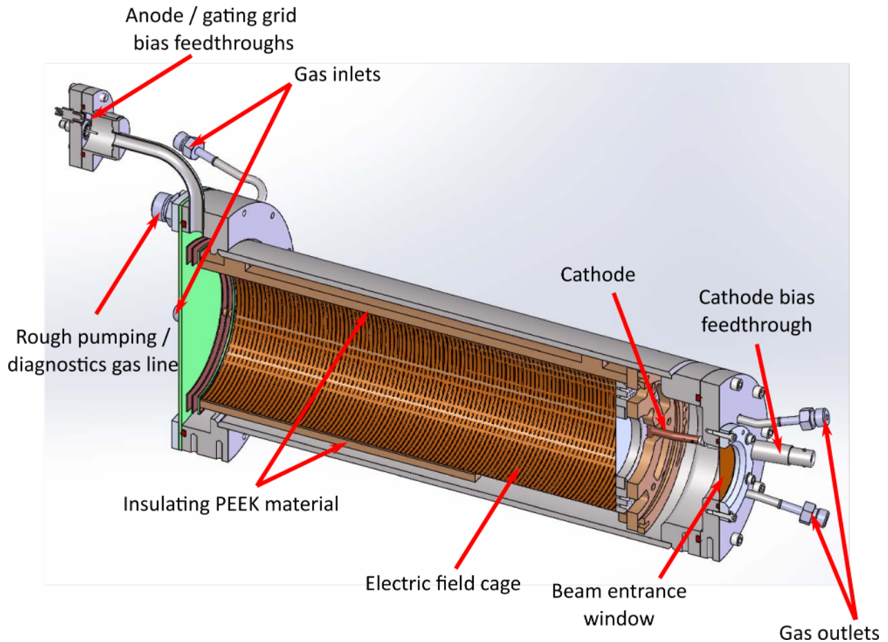
Figure 3.2: Mechanical design drawing of the Proton Detector.
