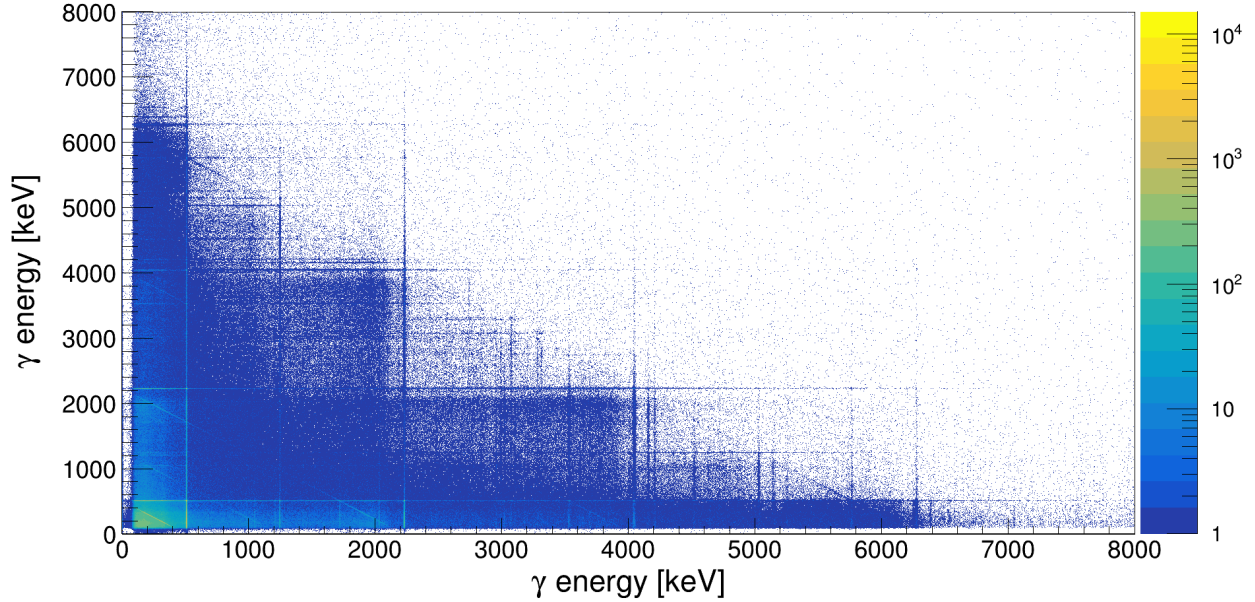
Figure 4.8: Two-dimensional \gamma - \gamma coincidence matrix for events occurring within the same 8\text{-}\mu\text{s} window preceding charged-particle radiation observed in the Proton Detector.
