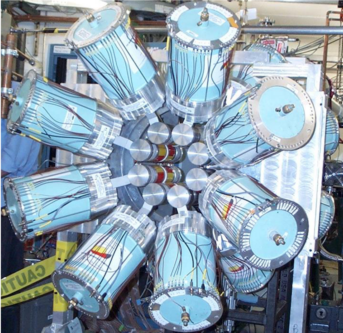
Figure 3.7: The betaSeGA, or “barrel,” configuration of the Segmented Germanium Array set up in the experimental vault. This employs 16 HPGe detectors in two rings around the beam line with a diameter of 17.3 cm. The large, blue-green containers are cryogenic storage dewars that hold the liquid N 2 for cooling the HPGe crystals located in the center of the array. Photo credit: National Superconducting Cyclotron Facility / Facility for Rare Isotope Beams, Dirk Weisshaar, Alexandra Gade.
