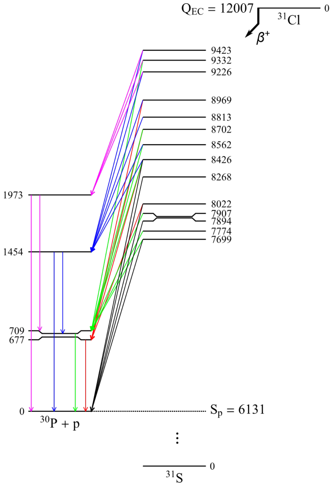
Figure 5.21: Preliminary, partial decay scheme for ^{31}\text{Cl}(\beta p \gamma)^{30}\text{P} , including only proton-unbound levels in ^{31}\text{S} that can result in a proton decay to a ^{30}\text{P} excited state.
