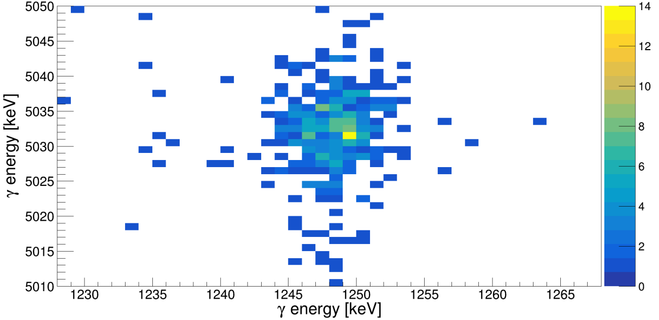
Figure 5.12: A two-dimensional histogram plotting \gamma - \gamma coincidences between the 1248- and 5030-keV transitions.
