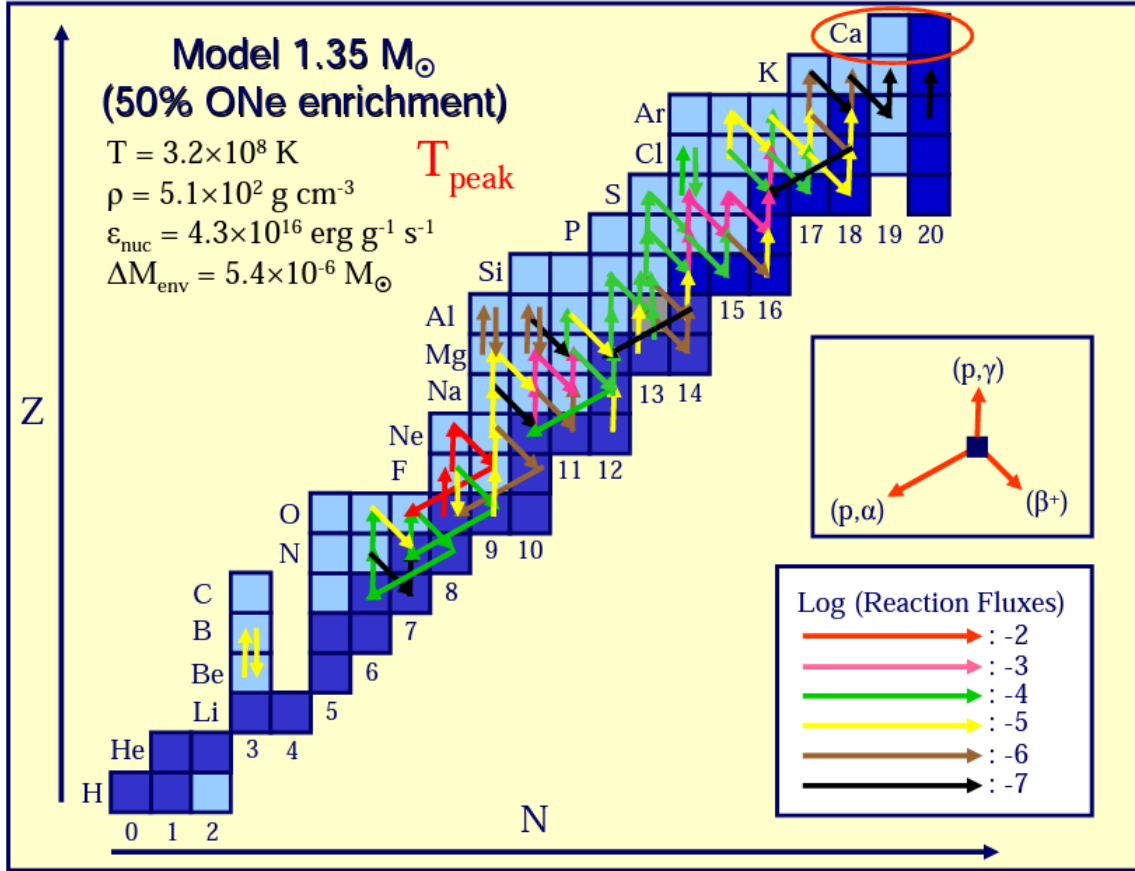
Figure 2.1: Path of nucleosynthesis in an ONe nova involving a 1.35- M_{\odot} white dwarf, assuming a 50% mixing ratio between the H-rich envelope and the underlying white dwarf material. Nuclides shown in dark blue are stable, while light blue squares correspond to radioactive nuclei. Figure credit: Ref. [59].
