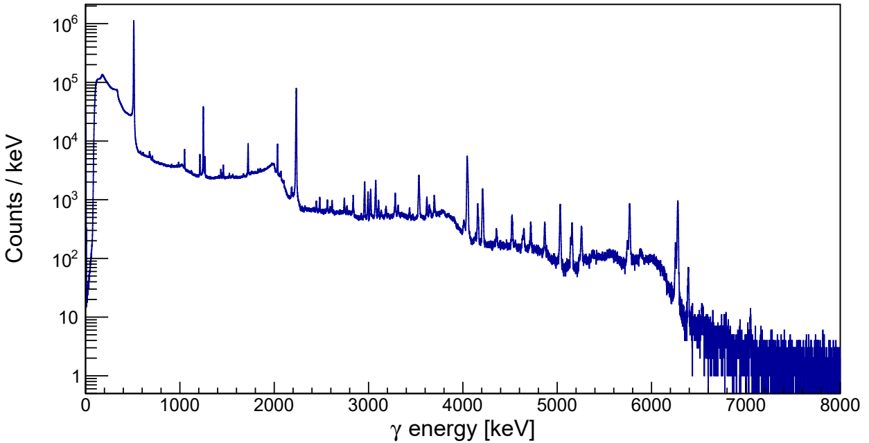
Figure 4.6: ^{31}\text{Cl} \beta -delayed \gamma ray singles spectrum including all events from 15 of the 16 SeGA detectors observed to be in coincidence with non-vetoed, charged-particle radiation in the Proton Detector.
