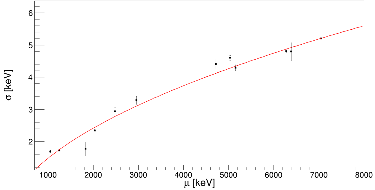
Figure 5.10: Peak width plotted with respect to peak position in the \gamma energy spectrum. The \chi^2 -minimized values of the free \sigma parameter are fit with a function proportional to the square root of the \mu parameter.
