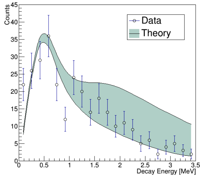
Figure 5.8: Solid lines represent theoretical spectra. The larger distribution (top line) assumes one neutron decay for all calculated ^{31}\text{Ne} states. The smaller distribution (bottom line) includes decays only from states in ^{31}\text{Ne} below S_{2n} = 3.72 \pm 1.62 MeV. The open markers indicate the measured spectrum. The only free parameter for this comparison is the overall scaling.
