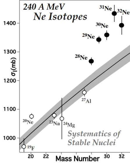
Figure 1.6: Interaction cross-sections \sigma_I reproduced from ref. [5]. Solid markers represent \sigma_I for neon isotopes with the solid line representing systematics of stable nuclei. Existing stable-nuclide data ( \sigma_I for ^{19}\text{F} , ^{24}\text{Mg} , ^{20}\text{Ne} and ^{23}\text{Na} and \sigma_R for ^{27}\text{Al} ) is shown in open markers.
