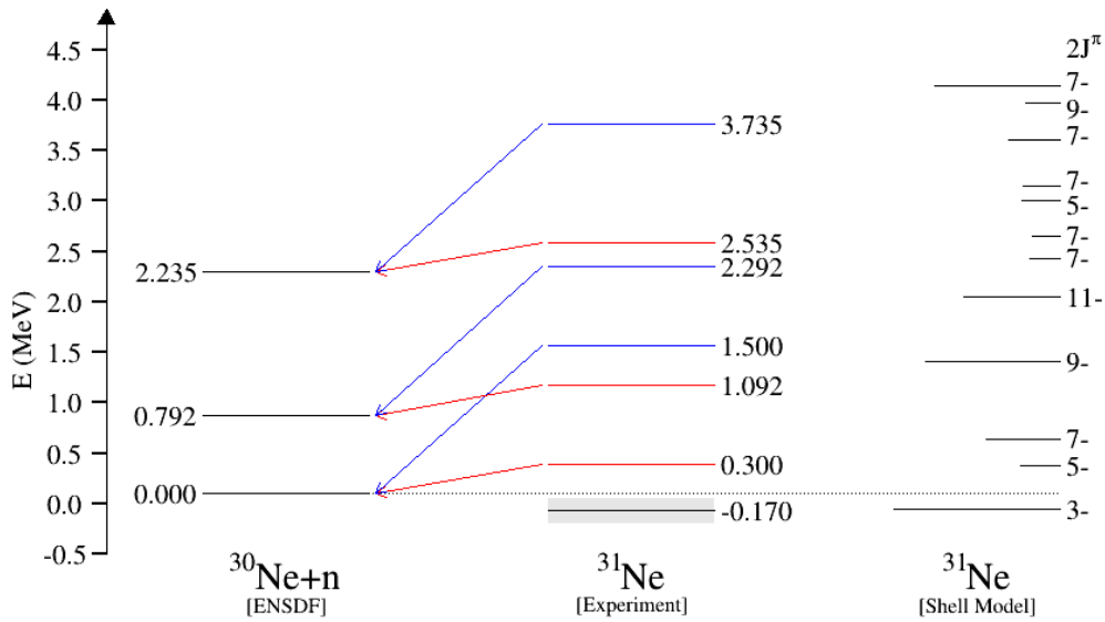
Figure 5.9: Decay energy and level scheme for the decay of ^{31}\text{Ne} into ^{30}\text{Ne} + n . The left level scheme shows states in ^{30}\text{Ne} from the Evaluated Nuclear Structure Data File (ENSDF). In the center are levels potentially observed by the present experiment, color coded by the measured decay energies (see text for detail). The arrows specify potential decay paths to states in ^{30}\text{Ne} . The right spectrum shows the NUSHELLX calculations with the length of the bars (excluding the ground state) indicating a population cross section from the two-proton knockout. Energies listed are relative to the one-neutron separation energy of ^{31}\text{Ne} .
