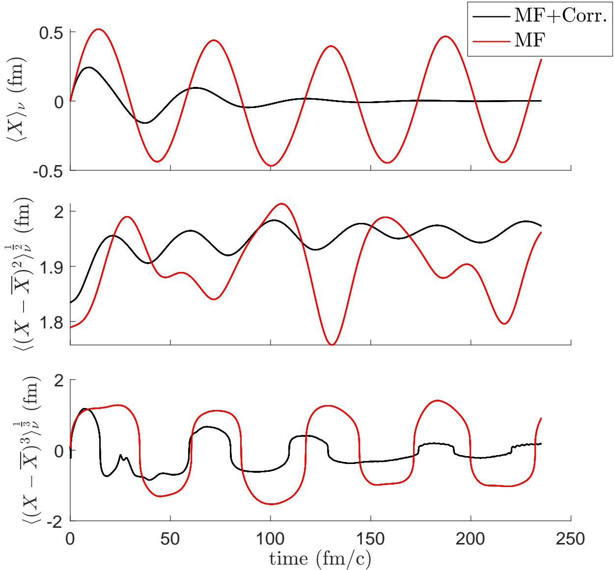
Figure 5.7: Evolution of the lowest three moments of the neutron slab. The red lines and the black lines correspond to calculations with mean field only and the full calculations, respectively.
