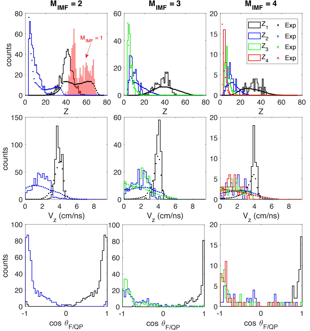
Figure 4.2: Charge Z (uppermost panels), parallel velocity V_z (middle panels) and angular \theta_{F/QP} distributions for the Ta+Au system at 39.6 MeV/nucl. The columns correspond to events of different IMF multiplicity M_{\text{IMF}} . Fragments are color-coded and sorted by their charge, with Z_1 being the heaviest and Z_{M_{\text{IMF}}} being the lightest. Simulation results are shown as histograms, and data of charge and velocity distributions extracted from Ref. [5] are shown as solid dots. The theoretical charge distribution of events with M_{\text{IMF}} = 1 is displayed as a semi-opaque shaded area in the background of the leftmost panel in the first row. (See the text for more discussion.)
