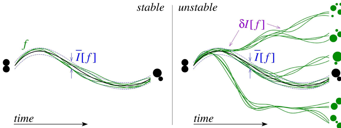
Figure 1.2: Schematic illustration of the effects of fluctuations in HIC. Under stable conditions without fluctuations on the left panel, the dynamical trajectories of identically prepared systems tend to be similar, leading to a unique outcome. The right panel shows that trajectories can spread out in the presence of fluctuations during the evolution and end up in diverse configurations. This figure is taken from [2].
