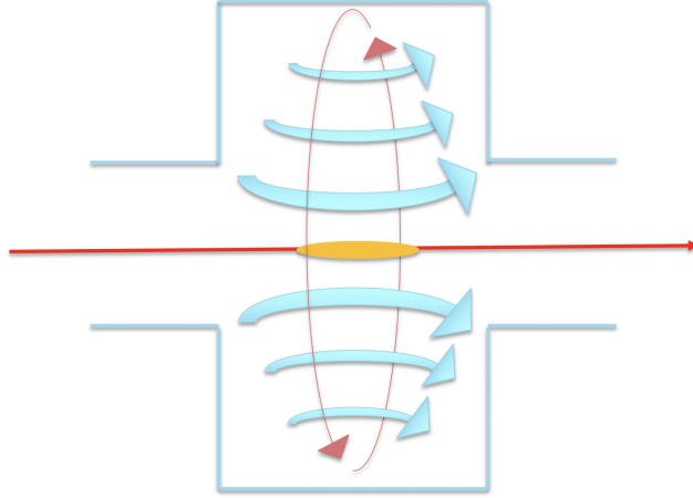
Figure 2.3: Full diagram depicting the longitudinal E field (blue) and the transverse magnetic field (red circulating) in the half phase in which a particle bunch (yellow) traverses the accelerating gap in the cavity.
