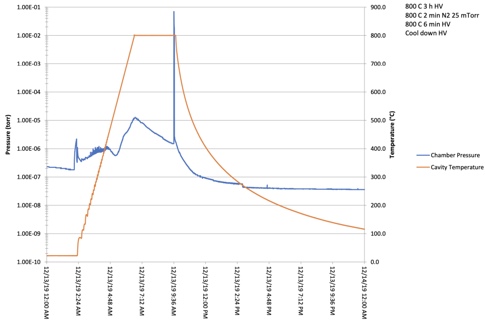
Figure 5.1: Time series gas pressure and temperature profile of the first 2/6 N-doping procedure conducted on S65-001 at FNAL.
