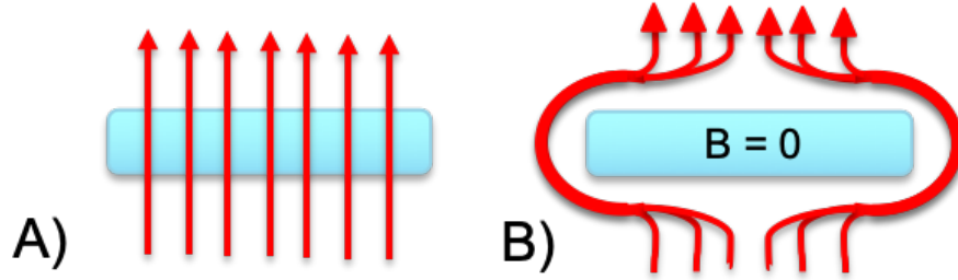
Figure 3.1: Drawing of the Meissner effect. An applied magnetic field (red) interacting with a superconducting material (blue) (A) at a temperature above T_c and (B) at a temperature below T_c .
