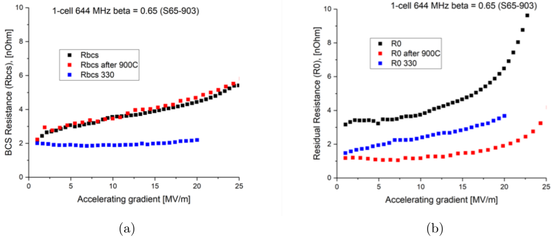
Figure 5.14: Deconvolution of R_0 and R_{BCS} showing the effect of 330^\circ\text{C} baking on each of these quantities in the 644 MHz single-cell prototype medium- \beta cavity. As expected, R_{BCS} is decreased significantly after the medium-temperature baking treatment, and the faintest hint of a reversal in field dependence of R_{BCS} also appears between 1 and 5 MV/m (a). Residual resistance is increased after the baking treatment (b).
