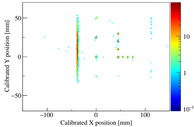
Figure 4.2: Result of the mask calibration of the downstream CRDC. The centroid of the charge distribution and the drift time of electrons were converted to the real position coordinates to reproduce the known positions of the holes or slits in the mask.
