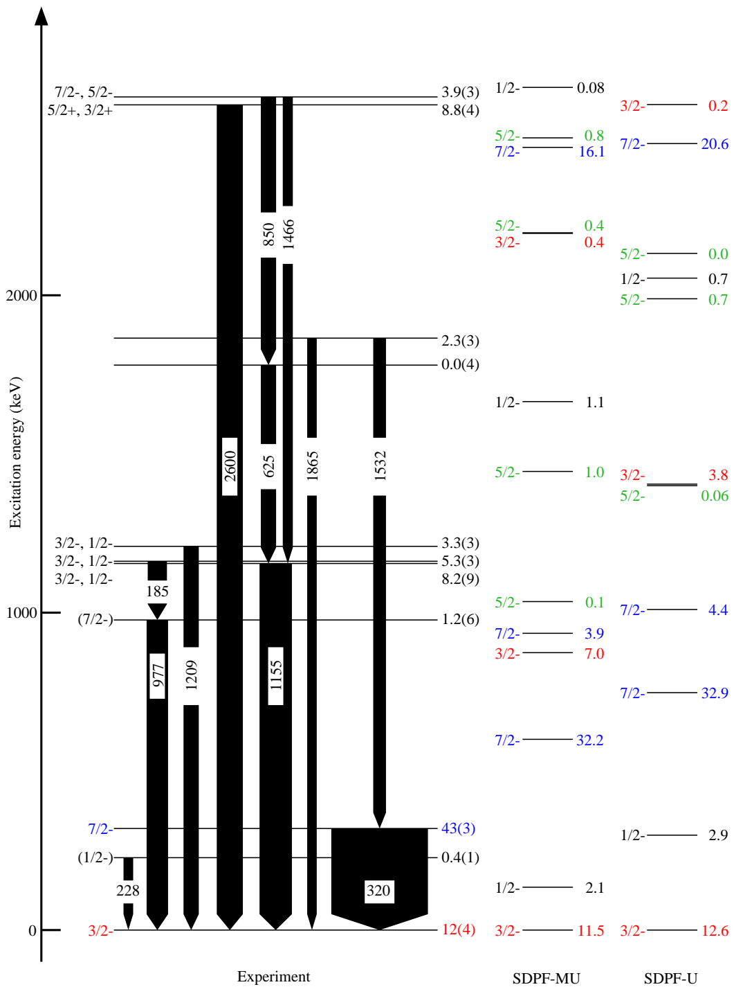
Figure 6.1: Level schemes of ^{43}\text{S} deduced from the present experiment and predicted by shell model calculations. In the experimental level scheme, observed \gamma -ray transitions are shown as arrows and their width reflect the \gamma -ray emission yield. In the experimental results and the shell model calculations, spin-parity and production cross section [mb] using Equation 2.47 of each state are presented. Spins and parities of 1/2^- , 3/2^- , 5/2^- , and 7/2^- are indicated in black, red, green, and blue, respectively.
