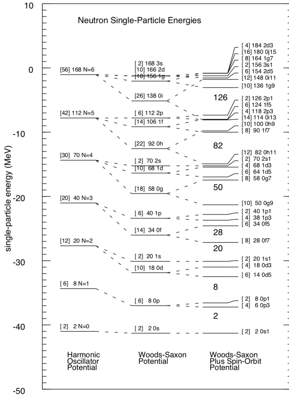
Figure 1.3: Example of the calculation of single-particle orbits. These calculations are for neutron single-particle states in ^{208}\text{Pb} with three different potentials. Taken from [5].
