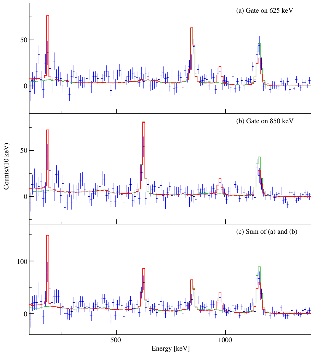
Figure 5.9: Comparison of \gamma - \gamma coincidence spectra with the simulation. (a) and (b) are the spectra gated on 625 and 850 keV transitions, respectively and (c) is the sum of (a) and (b). Blue points are the experimental data with addback. Red lines are simulated spectra assuming both 185 and 1155 keV transitions are coincident with the 850 \rightarrow 625 keV cascade. The branching ratio of the 185 and 1155 keV transitions was estimated from the singles spectrum. Green lines are also simulated spectra, this time assuming 100% branching ratio for 1155 keV and no coincidence with 185 keV transition. These red and green histograms correspond to the scheme 1 and 2 in Figure 5.8, respectively.
