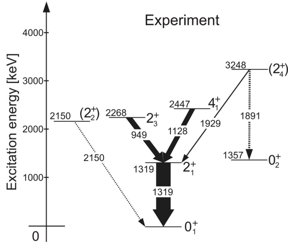
Figure 1.5: Level scheme of ^{44}\text{S} constructed by [19]. Through the comparison with the shell model calculation, the ground state band (the 0_1^+ and 2_1^+ states) is considered to be the 2p2h neutron intruder configuration with the prolate deformation, though the 0_2^+ state is the 0p0h normal configuration with the spherical shape. The 4_1^+ state is thought to be the K = 4^+ isomeric state of 1p1h configuration.
