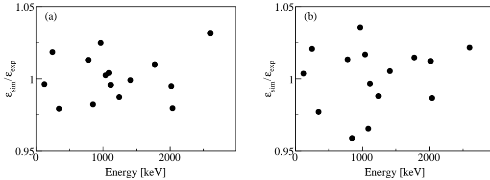
Figure 4.14: Ratio of simulated and measured efficiencies of GREYINA. Figure (a) and (b) are the plots without and with addback.
