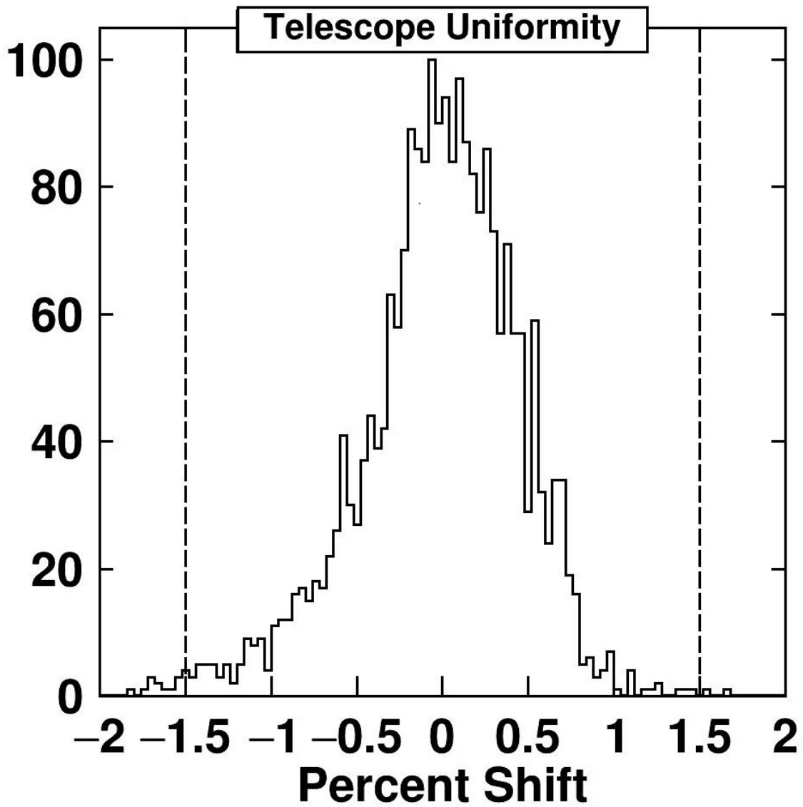
Figure 2.15: Percent Shift Percent shift for all points in all telescopes. It can be seen from this figure that nearly every point lies within the +/- 1.5 percent shift that was specified for the HiRA10 crystals.
