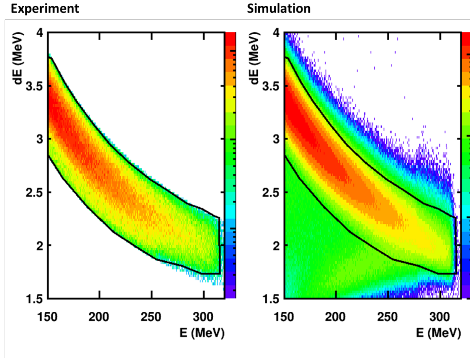
Figure 5.30: Triton PID Gate Left: PID gate around experimental data. Right: PID gate around simulated data.
