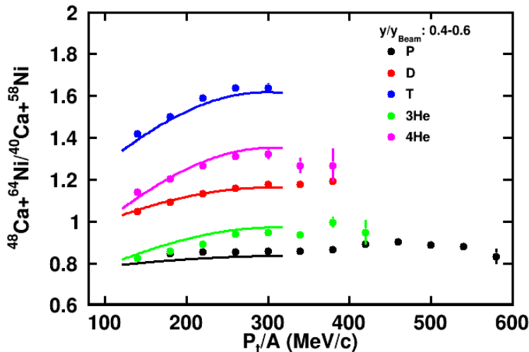
Figure 6.21: Isoscaling Ratios Shows Isoscaling ratios created for P, D, T, ^3\text{He} and alphas. The lines over the different isoscaling ratios come from the extracted chemical potentials. Where in this case the chemical potentials were created by fitting both the measured particles and their combinations.
