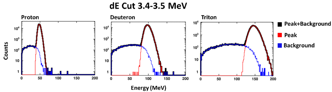
Figure 5.2: dE Cut Simulated PDT Data Panels show a dE cut from 3.4-3.5 MeV on the simulated data. The red lines indicate particles considered to be in the peak and the blue the background.
