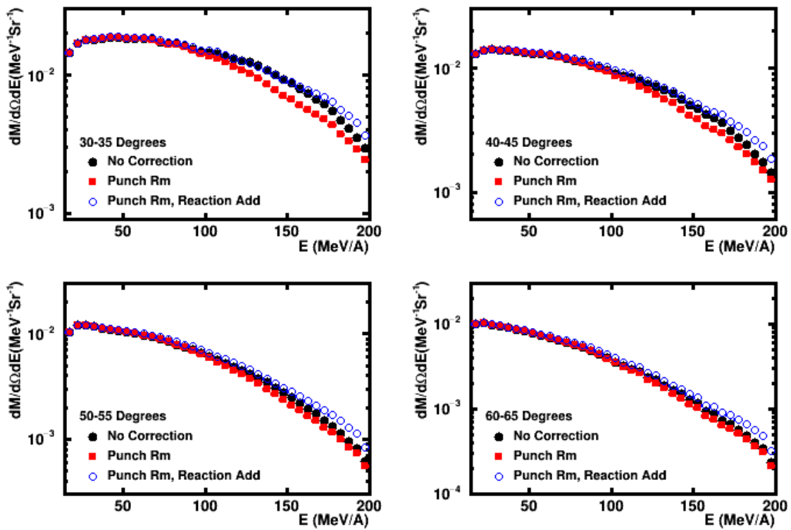
Figure 6.12: Comparison of proton energy spectra for ^{40}\text{Ca}+^{58}\text{Ni} The black points are for data without the punch-through or reaction loss correction. Red points show data that has been corrected for punch-through and blue points show the data after both punch-through and reaction losses have been corrected.
