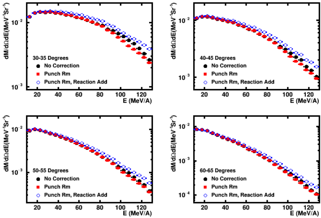
Figure 6.14: Comparison of deuteron energy spectra for ^{40}\text{Ca} + ^{58}\text{Ni} . The black points are for data without the punch-through or reaction loss correction. Red points show data that has been corrected for punch-through and blue points show the data after both punch-through and reaction losses have been corrected.
