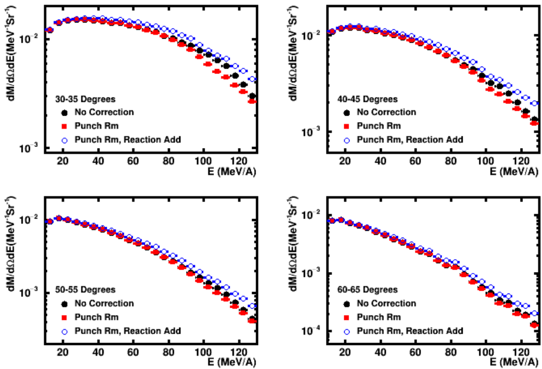
Figure 6.13: Comparison of deuteron energy spectra for ^{48}\text{Ca} + ^{64}\text{Ni} . The black points are for data without the punch-through or reaction loss correction. Red points show data that has been corrected for punch-through and blue points show the data after both punch-through and reaction losses have been corrected.
