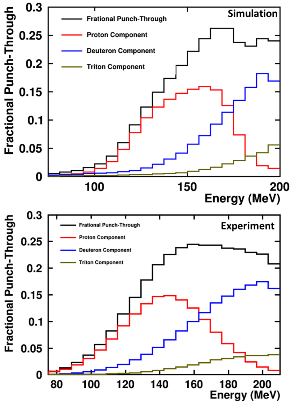
Figure 5.58: Fractional Punch-Through Contamination Protons Telescope 2 Top: Fractional punch-through contamination within the proton PID line estimated by NPTTool simulations. Bottom: Fractional punch-through contamination with the proton PID line as estimated by the above analysis.
