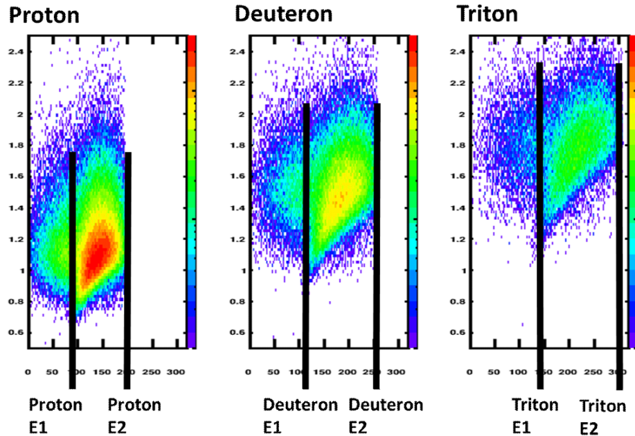
Figure 5.49: Simulated Punch-Through Tails The black vertical lines indicate the range in E over which the simulated punch-through tails exist.
