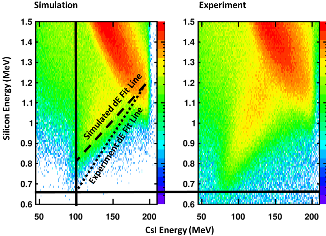
Figure 5.41: Simulated and Experiment Proton PID with Punch-Through Tail Right: PID for experimental Proton data for telescope 2. The black line at the bottom indicated the lowest dE point in the punch-through tail. Left: PID for simulated Proton data for telescope 2. The solid black horizontal line indicated the minimum dE for the punch-through tail in the experimental data. The vertical solid black line indicates the lowest value in E that the simulated punch-through tail is observed at. The thick dashed line is the fit from (E_{CsIPunch}, E_{SiliconPunch}) to (E_{CsIMinPunchTailSim}, E_{SiliconMinPunchTailSim}) . The thin dashed line is fit from (E_{CsIPunch}, E_{SiliconPunch}) to (E_{CsIMinPunchTailSim}, E_{SiliconMinPunchTailExp}) .
