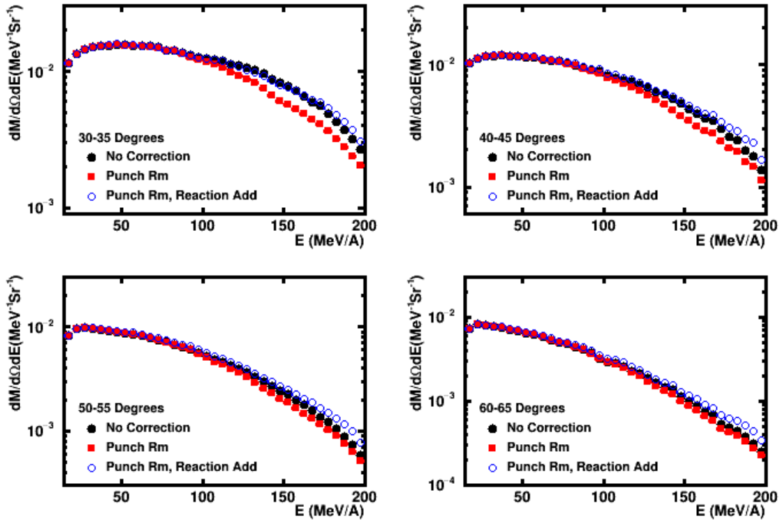
Figure 6.11: Comparison of proton energy spectra for ^{48}\text{Ca}+^{64}\text{Ni} The black points are for data without the punch-through or reaction loss correction. Red points show data that has been corrected for punch-through and blue points show the data after both punch-through and reaction losses have been corrected.
