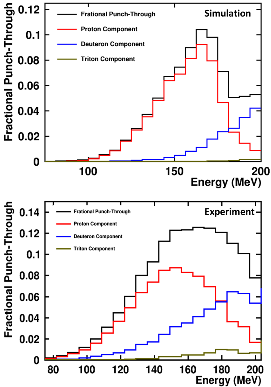
Figure 5.60: Fractional Punch-Through Contamination Protons Telescope 9 Top: Fractional punch-through contamination within the proton PID line estimated by NPTTool simulations. Bottom: Fractional punch-through contamination with the proton PID line as estimated by the above analysis.
