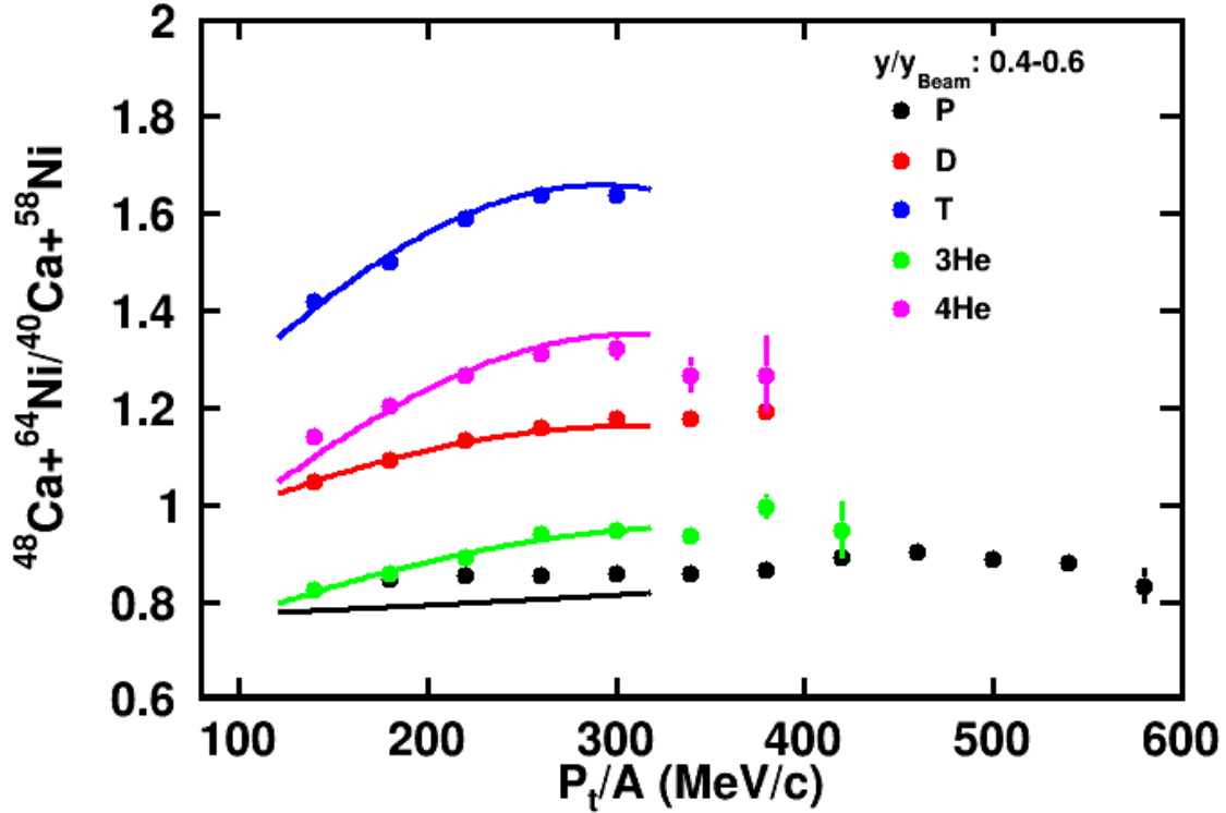
Figure 6.30: Isoscaling Ratios Shows Isoscaling ratios created for P,D,T, {}^3\text{He} and alphas. The lines over the different isoscaling ratios come from the extracted chemical potentials. Where in this case the chemical potentials were created by fitting both the measured particles and their combinations however protons and combinations created with protons were all left out.
