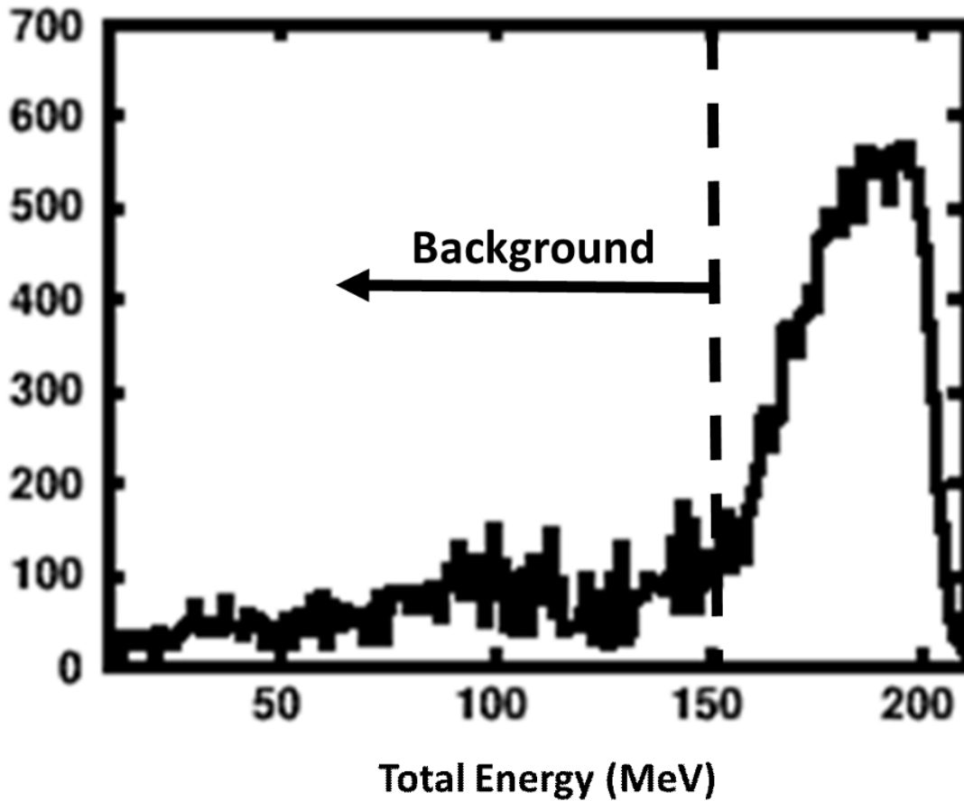
Figure 5.42: dE Cut 1.1-1.15 MeV with Punch-Through Removed This figure shows a dE cut post punch-through subtraction. The dashed line indicates the boundary placed to distinguish between what is considered background as compared to good events that fully deposit their energy.
