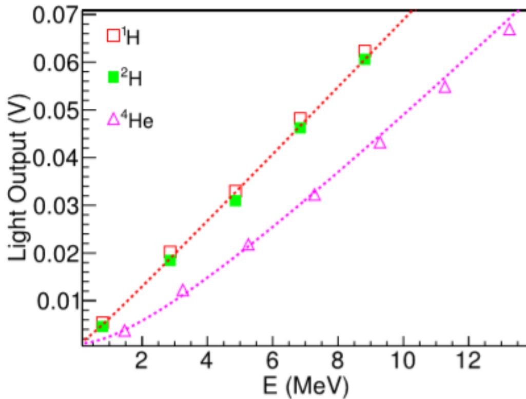
Figure 4.12: Low Energy Calibration Points CsI light output as a function of incident energy. Proton are shown as red squares, deuterons as green squares and alphas as pink triangles. [45]
