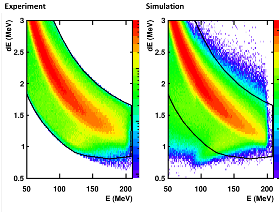
Figure 5.28: Proton PID Gate Left: PID gate around experimental data. Right: PID gate around simulated data.
