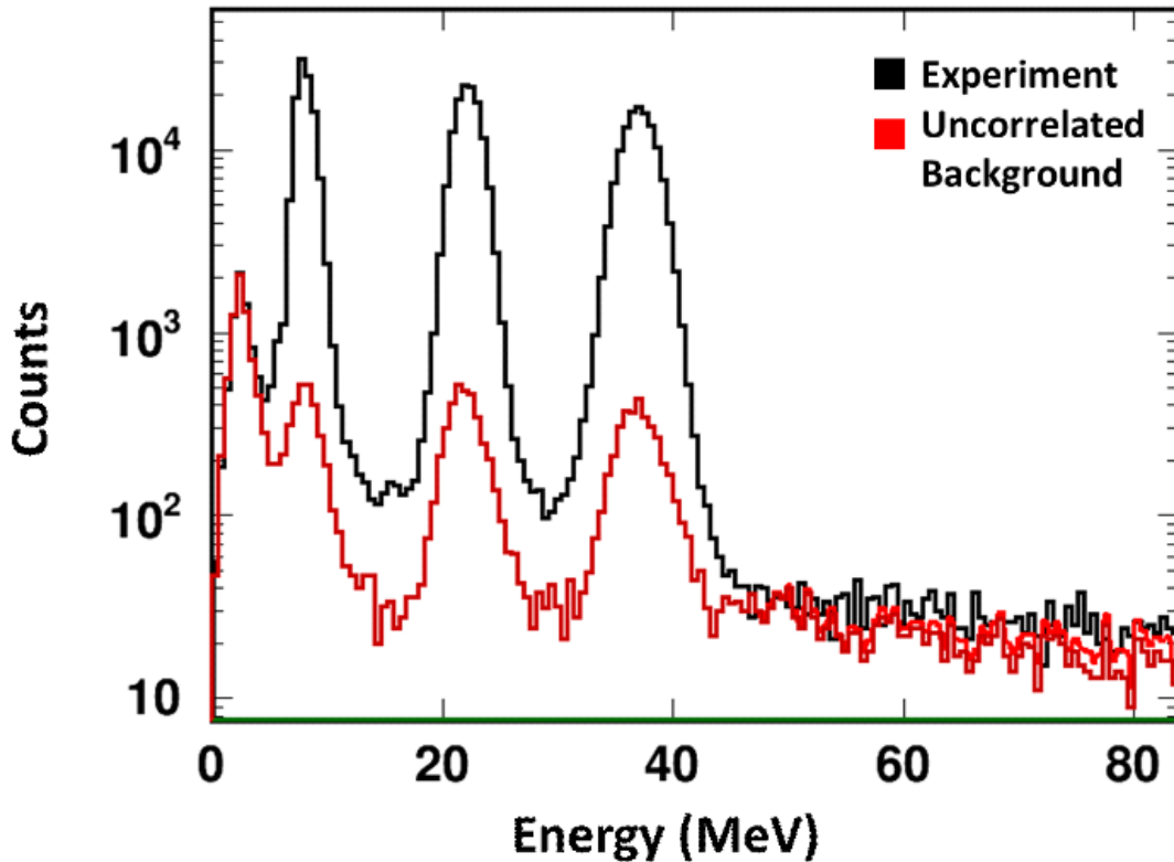
Figure 5.9: dE Cut with Total Uncorrelated Background Spectra Plotted dE cut from 10-10.25 MeV. The black line shows the experimental data while the red shows the estimated uncorrelated background. The uncorrelated background is created by adding the Type 1 uncorrelated background to the Type 2 uncorrelated background
