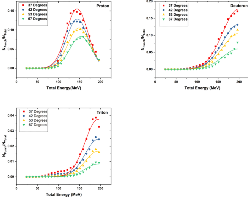
Figure 5.54: Fit on Relative Punch-Through 3 Panels show relative punch-through contamination within the proton PID cut at different angles for protons, deuterons and tritons. These fits were used to create equations as functions of angle and energy for removing the punch-through from beneath the proton PID line. Additional functions were made to describe deuterons and tritons.
