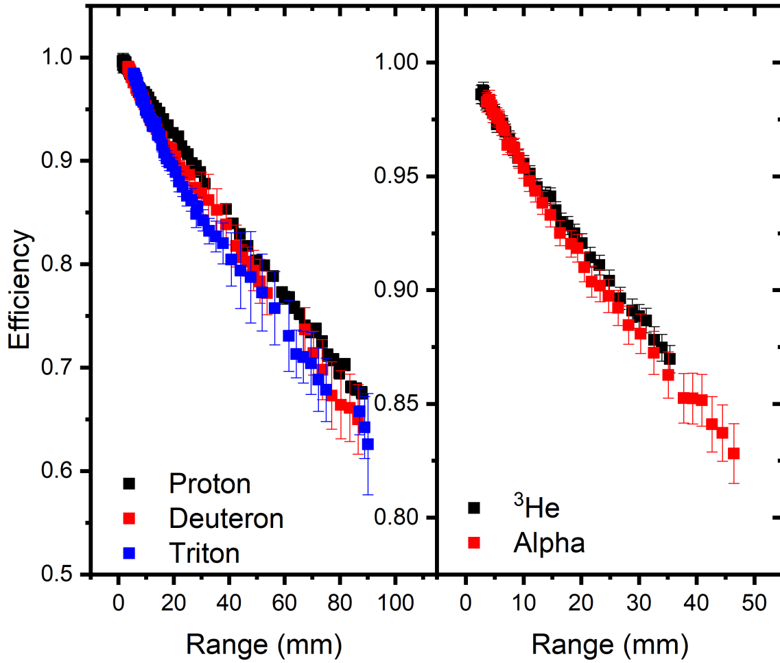
Figure 5.15: Light Charged Particle Efficiencies Range vs efficiency plots for protons, deuterons, tritons, 3 He and alpha particles.
