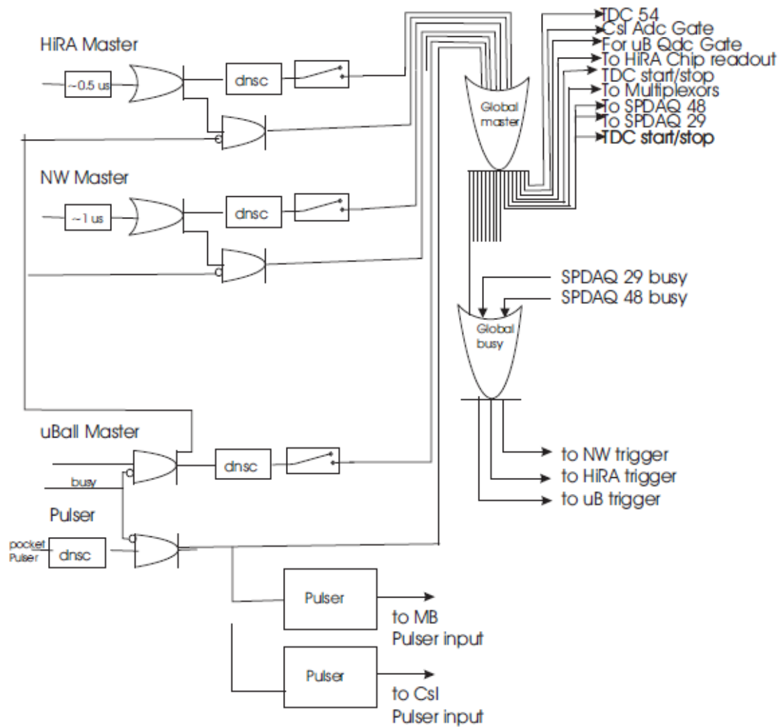
Figure 3.11: Experiments 14030 and 15190 Master Trigger
